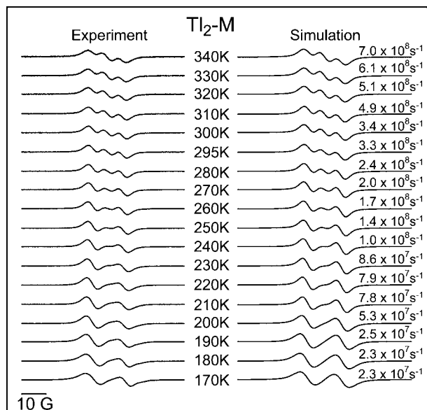
Figure 4. Variable-temperature EPR spectra of the monocation of Tl_2-M (left) and simulated spectra (right) with derived hole-transfer rates.
