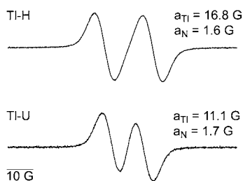
Figure 2. Room-temperature EPR spectra of the monocations of TI-U and TI-H .
