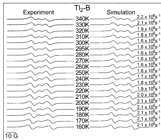
Figure 5. Variable-temperature EPR spectra of the monocation of Tl_2-B (left) and simulated spectra (right) with derived hole-transfer rates.
