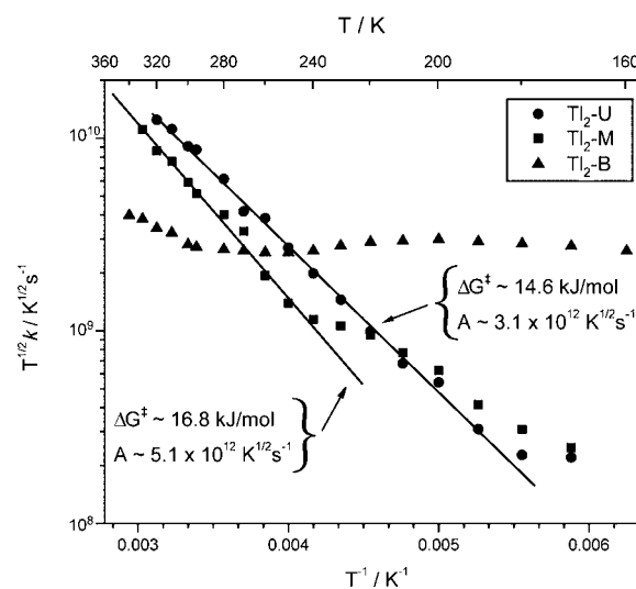
Figure 6. Marcus-equation plots for the monocations of Tl_2-U , Tl_2-M , and Tl_2-B .
