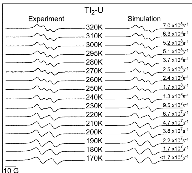
Figure 3. Variable-temperature EPR spectra of the monocation of Tl_2-U (left) and simulated spectra (right) with derived hole-transfer rates.
